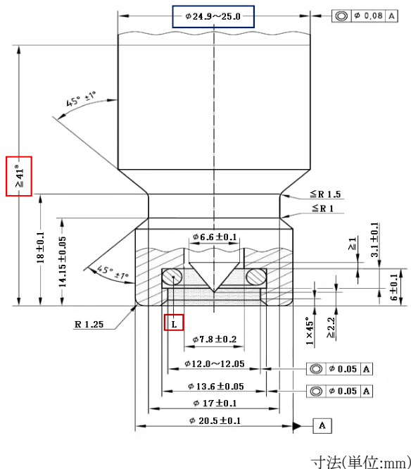
図 1: M1 および N1 車両の 20 MPa 充填装置 (レセプタクル) Figure 1: 20 MPa filling unit (receptacle) for M1 and N1 vehicles
