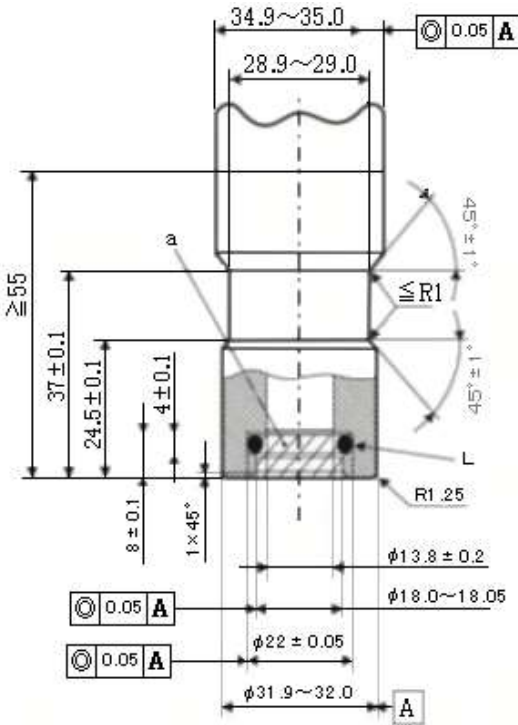
Figure 2: 20 MPa Filling unit Size 2 (receptacle) for M2, M3, N2 and N3 vehicles
